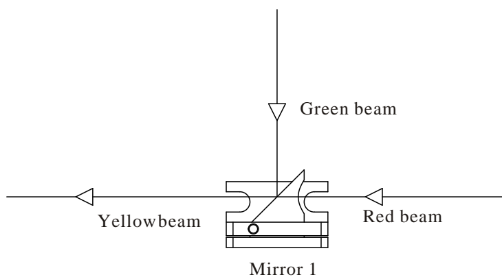
Fig7-2 RGY laser beams mix system
